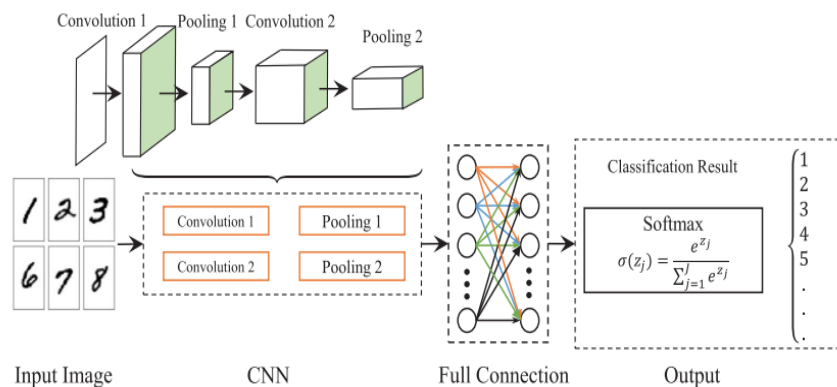
Figure 2. CNN model
