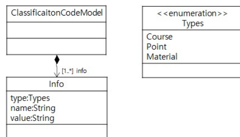
Fig. 4. ClassificationCode Metamodel
