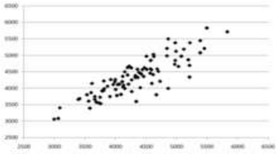
Fig 2. A Linear Regression Model for Prediction of Heat Demand in Winter
