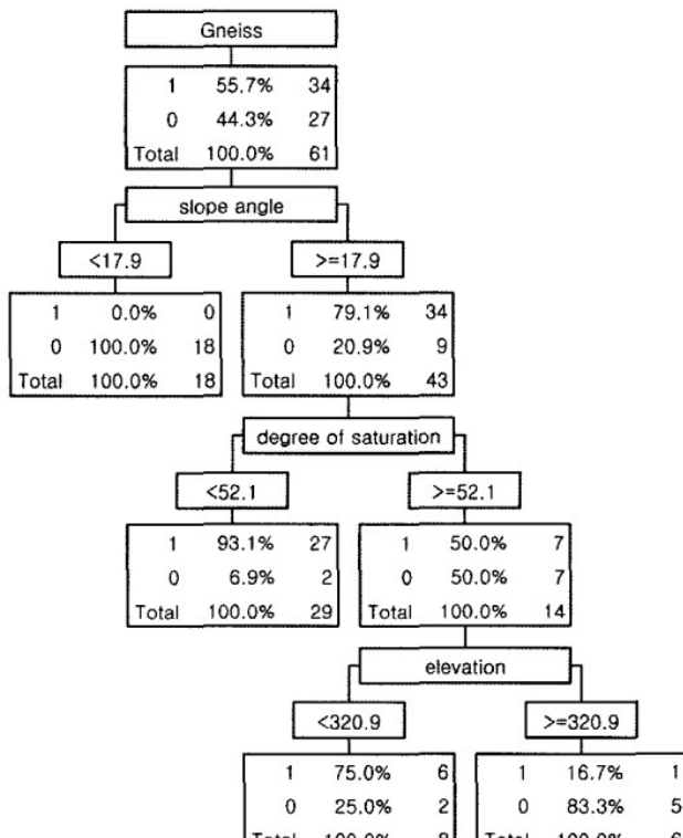
Fig 3. Decision tree for prediction between steep and non-slope areas
