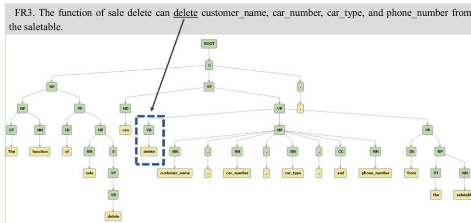
Figure 2. Morphological Analysis of the Functional Requirement
