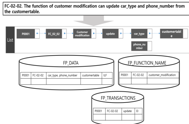
Figure 3. DB tables of Requirements
