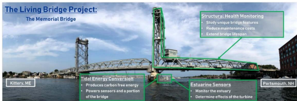
Figure 2. Structural Health Monitoring System Project on Memorial Bridge, United States
