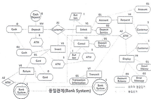
Fig. 10. Case Relation
